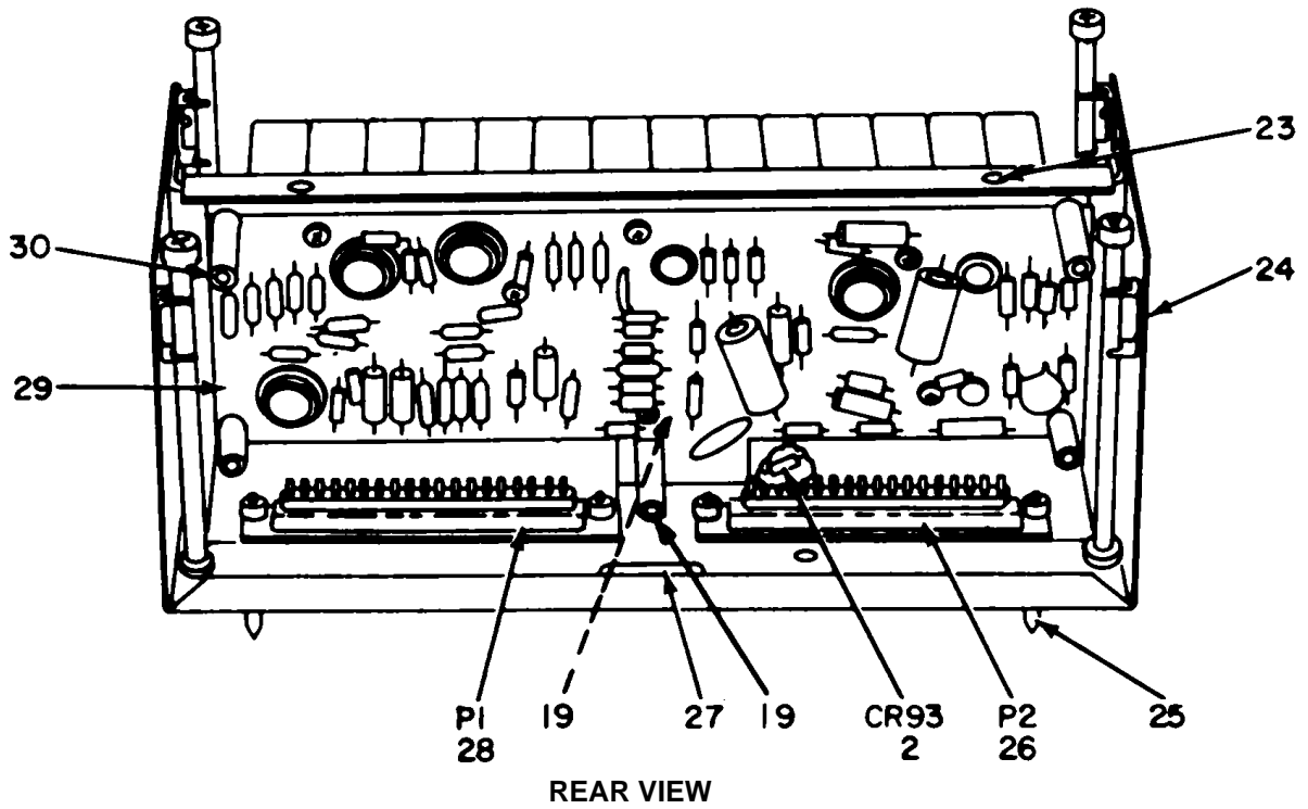
Figure 4. Control, Antenna Coupler (A2) (Sheet 2 of 2).
